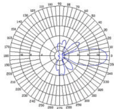
E-Plane Field Pattern
